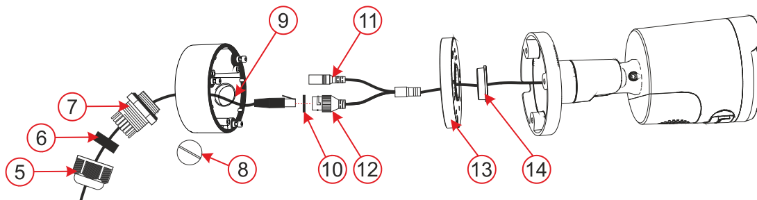
Fig. 3: Installation procedure using the mounting socket
